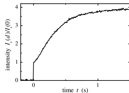
Fig. 2. Temporal dynamics of the transmitted signal beam measured for total light intensity I = 30 \text{ mW/cm}^2 , beam ratio \beta = 80 , applied field with amplitude V_0 = 2.6 \text{ V} , and frequency f = 20 \text{ kHz} at grating spacing \Lambda = 440 \mu\text{m} . The pump beam continuously illuminates the LCLV, and the signal beam is unblocked at t = 0 .
